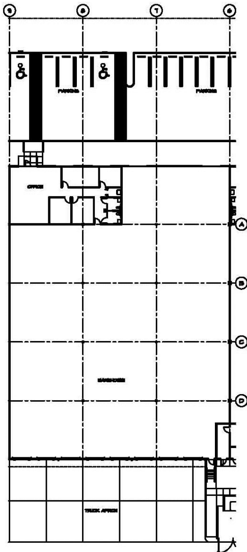
GENERAL FLOOR PLAN SCALE: 1/8" = 1'-0"
